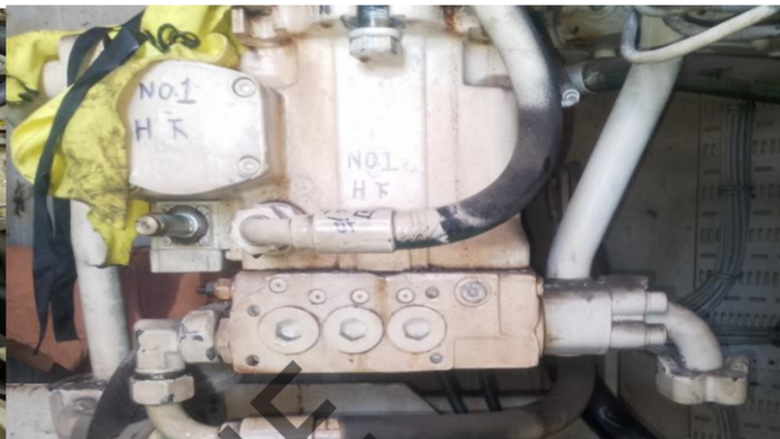
Made marks before dismantle the pumps to avoid wrong matching
